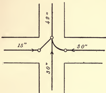
FIG. 4.—ALIGNMENT OF SEWER-JUNCTIONS.
